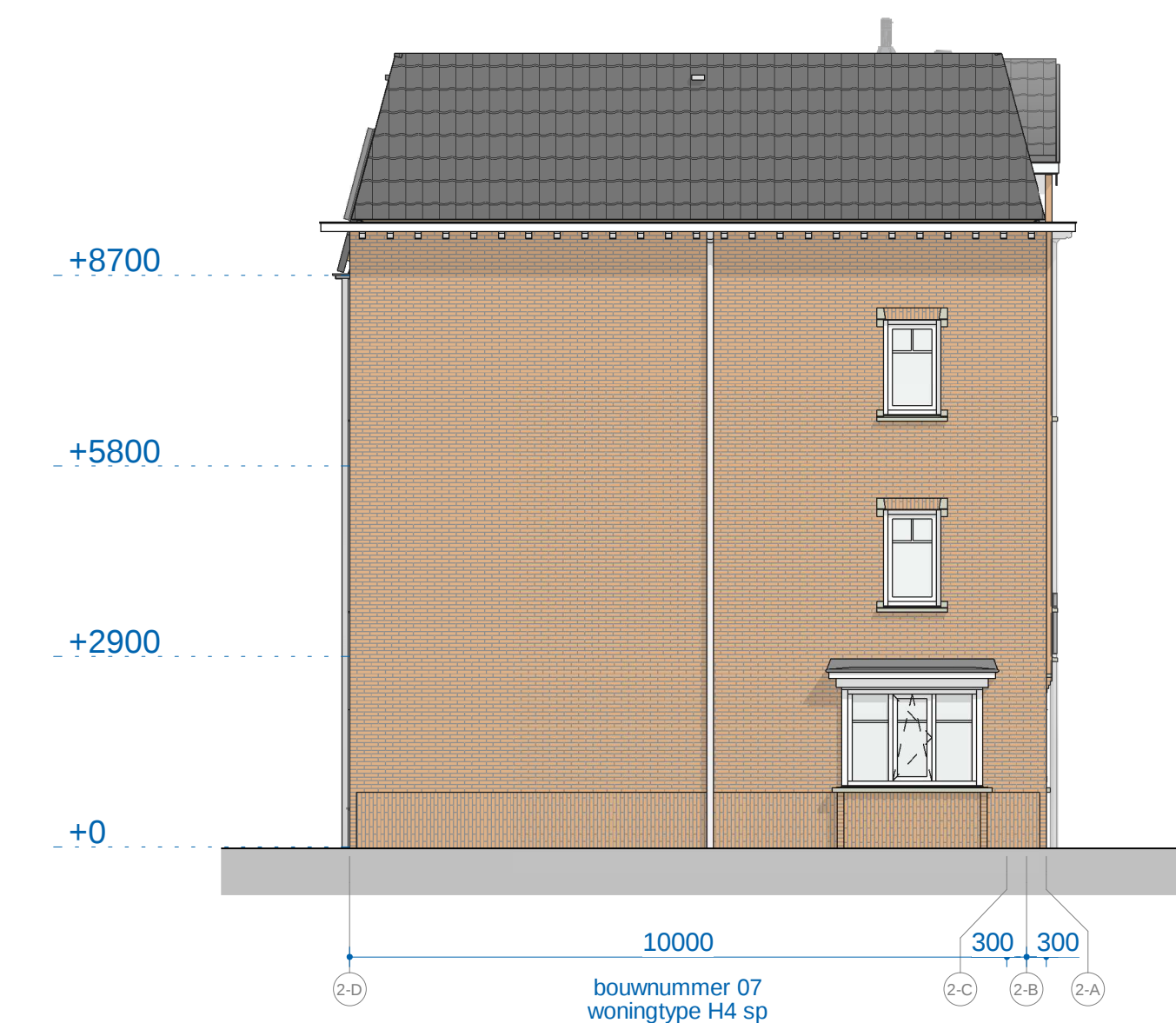
B2_linkergevel
